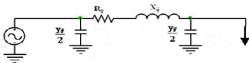
Figure 1: π circuit model of a transmission line
