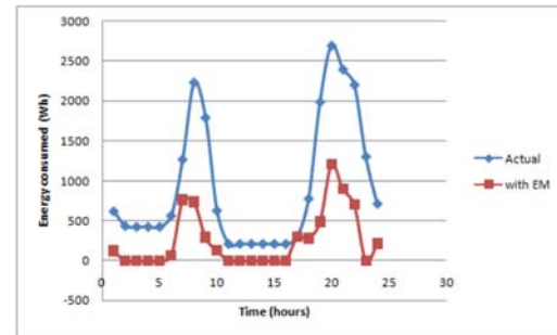
Fig. 6: Comparison plot of actual and proposed system
