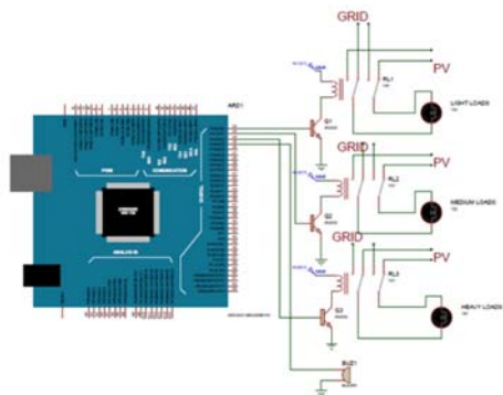
Fig.7: System architecture
