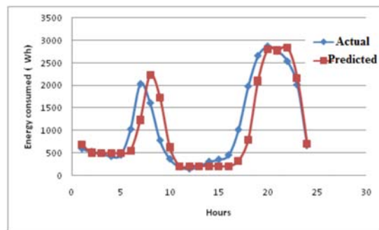
Fig.3: Comparison plot of load prediction
