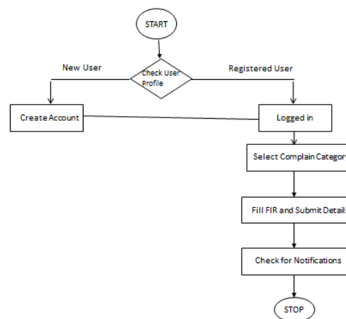
Figure 4.2 Flow graph for User
