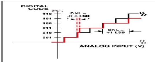
Figure 1a. DNL error: no missing codes
