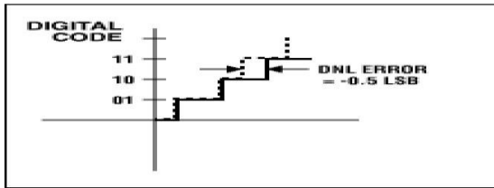
Figure 1b. DNL error: no missing codes
