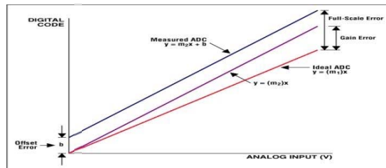
Figure 5. Offset, gain, and full-scale errors
