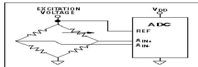
Figure 8. Ratiometric ADC conversion
