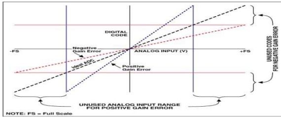
Figure 6. Gain error reduces dynamic range.
