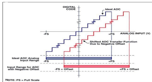
Figure 2. Bipolar offset error
