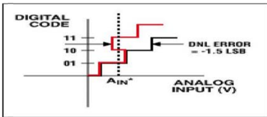
Figure 1d. DNL error: At A_{IN^*} , the digital code can be one of three possible values. When the input voltage is swept, Code 10 will be missing.
