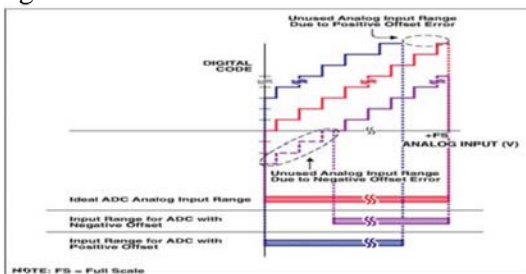
Figure 4. Unipolar offset error
