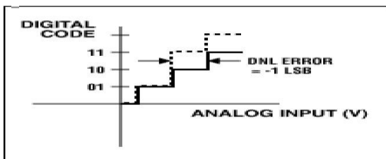
Figure 1c. DNL error: Code 10 is missing
