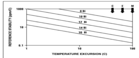
Figure 7. Voltage-reference-drift requirements relate to ADC resolution.
