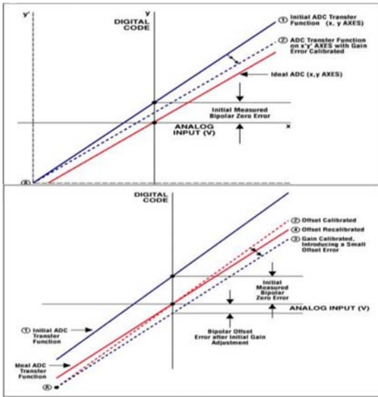
Figures 3a and 3b. Calibrating bipolar offset error. (Note: The stair-step transfer function has been replaced by a straight line, because this graph shows all codes and the step size is so small that the line appears to be linear.)
