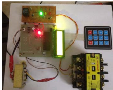
Fig: CB in closed state shown by green LED
