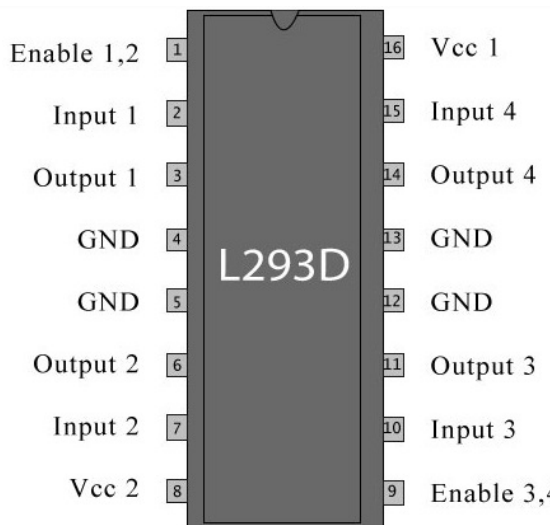
Fig 4: Pin Diagram of L293D
