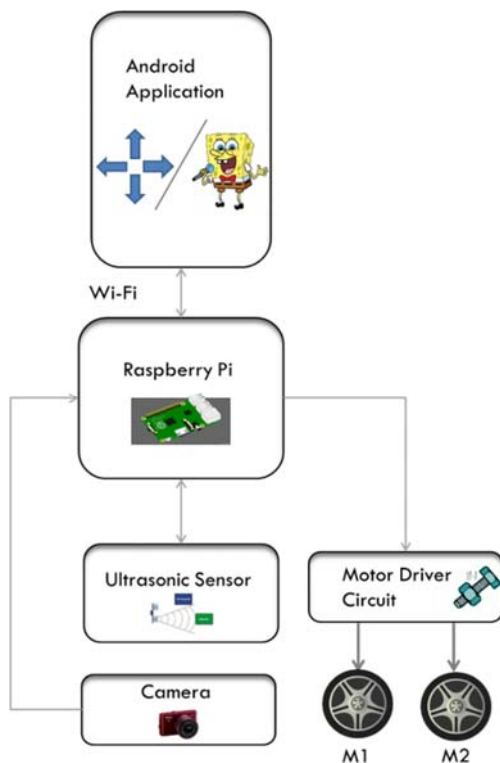
Fig 1: Block Diagram
