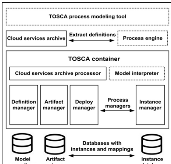
FIGURE 7. Sample architecture of a TOSCA cloud environment. Indeed,
