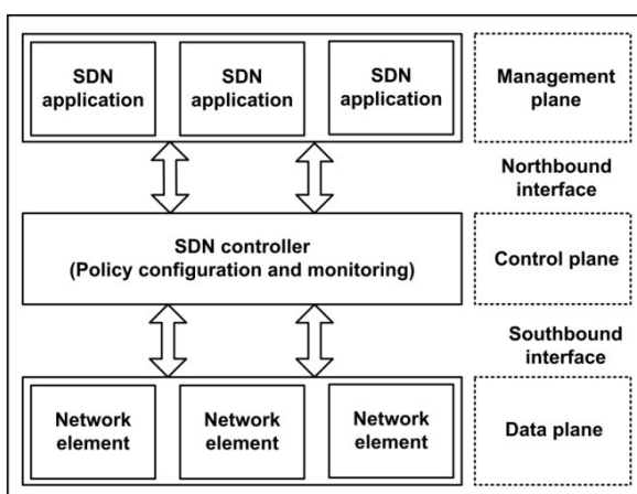
FIGURE 2. System architecture of software defined networks.
