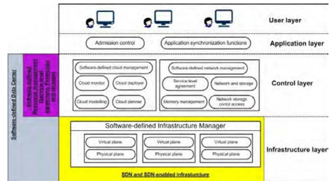
FIGURE 1. (a) SDCC administration model. (b) Major components of SDCC.
