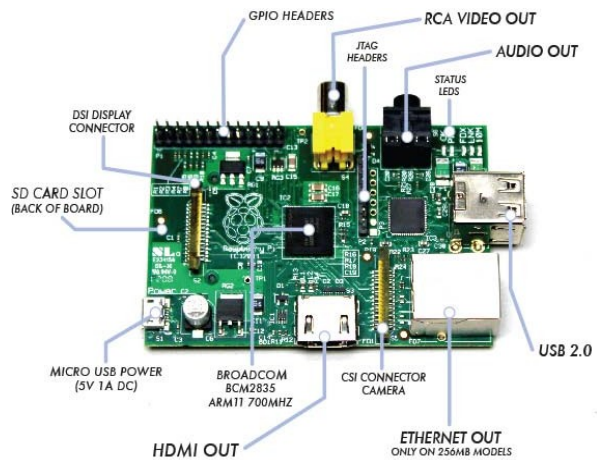
Fig. 2. Raspberry Pi
