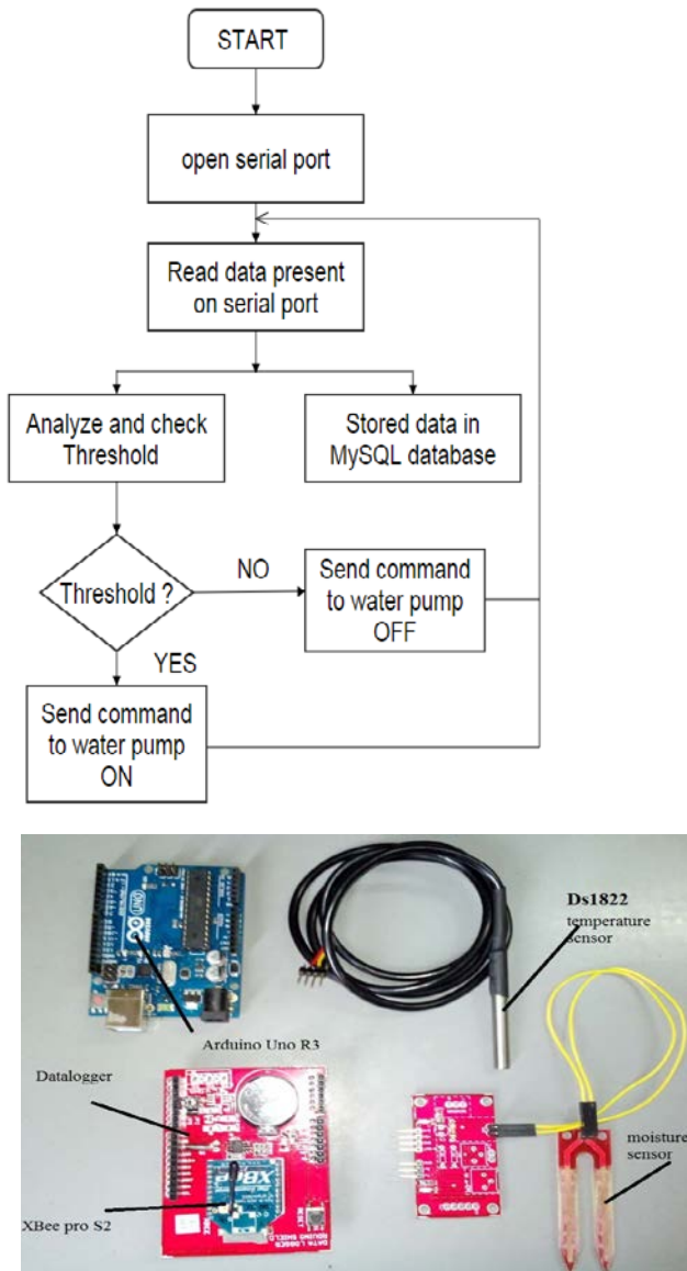
Fig. 5. Coordinator node flowchart
