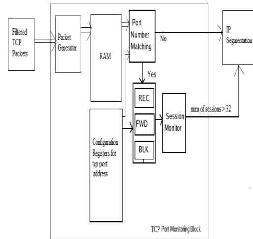
Figure. 4 TCP Port Monitoring System
