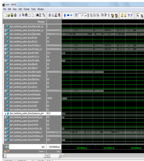
Figure. 7 Packet Blocking
