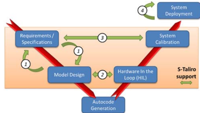
Figure 2: Testing Processor Stages
