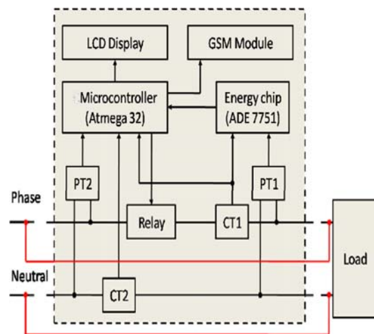
Fig : 7 : Bypassing of whole meter
