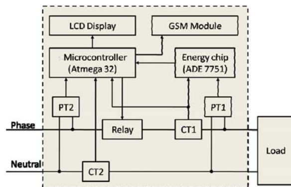
Fig : 3 : Block diagram of the GSM based smart meter.
