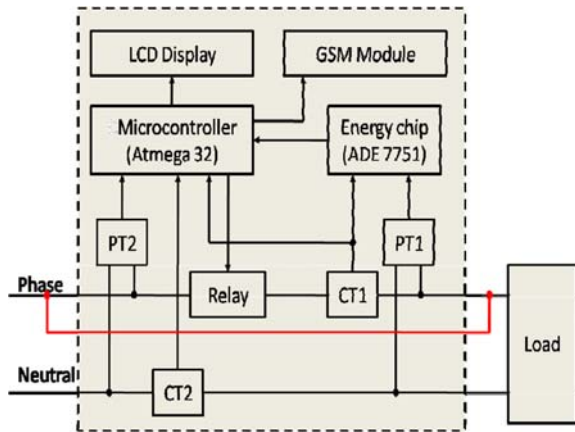
Fig : 5 : To bypass conventional meter is shorting the phase line
