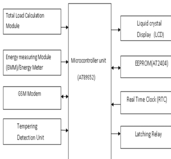
Fig : 4 : Block diagram of GSM based AMR
