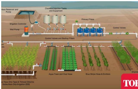
Figure 1: Drip Irrigation System using WSN
