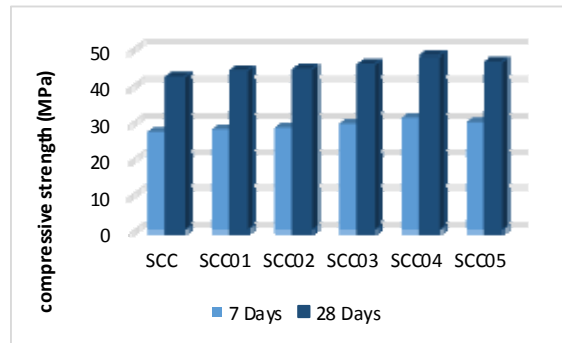
Fig-5.2: Compressive strength of Self Compacting Concrete
