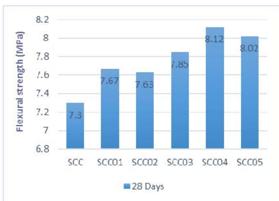
Fig-5.4: Flexural strength of Self Compacting Concrete
