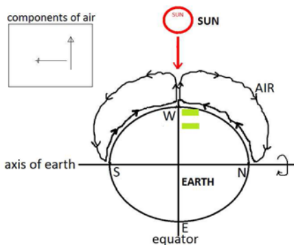
Fig. 3. Global air, with including the rotation of earth
