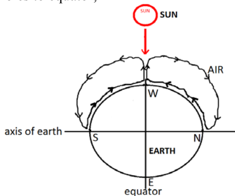
Fig. 2. Global air, with earth assumed stationary
