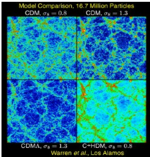
Figure 5 Simulation: Comparison of four astrophysical N-body Cold Dark Matter Model variants.
