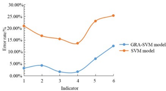
Figure 4: Comparison of error rates between GRA-SVM based prediction model and SVM based prediction model
