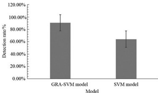
Figure 5: Comparison of detection rate between GRA- SVM based prediction model and SVM based prediction modelthe SVM based prediction model in terms of overall de- tection coverage and average detection time. So it can be said that GRA-SVM based prediction model is relatively efficient and more suitable for the practical application of network security issues
