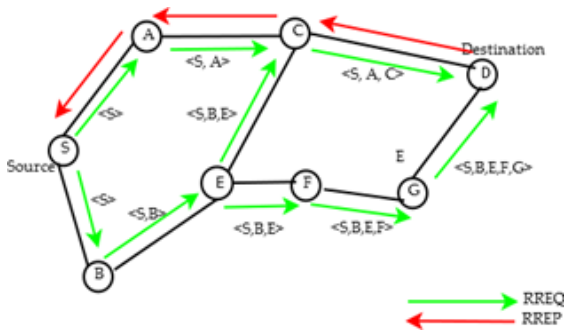
Fig. 1: Route Exploration in AODV protocol
