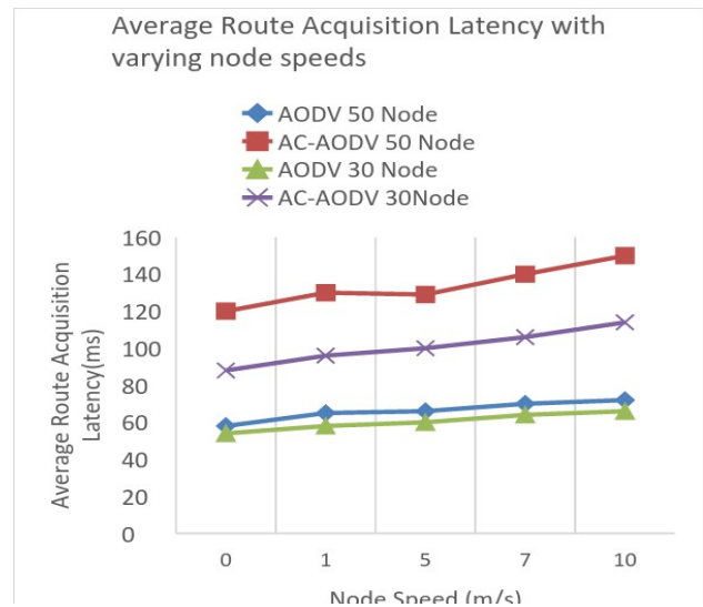
Fig.6: Average Route Acquisition Latency with varying node speeds
