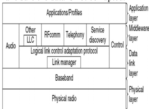
Figure 1 Bluetooth Stack
