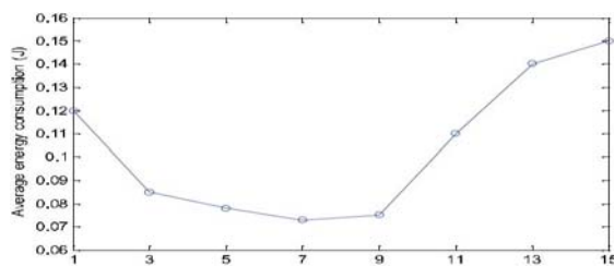
FIGURE 9. Average energy consumption with different m .
