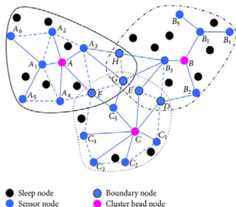
Figure 1: Clustering in a sensor network
