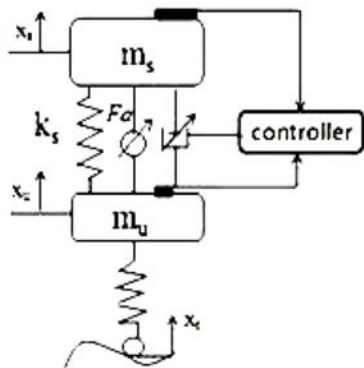
Fig.6. Active Suspension System
