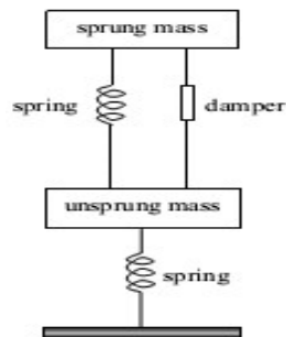
Fig 2 Quarter Car Passive Suspension System.
