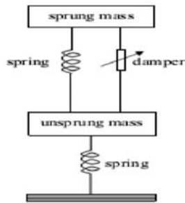
Fig 3 Quarter Car Semi-active Suspension System
