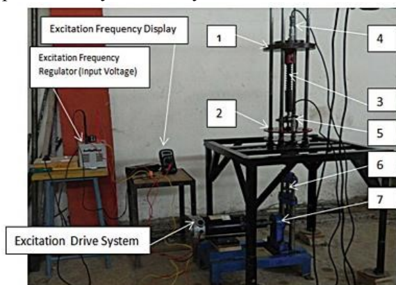
Fig.7. 2 DOF-QC-PSS Model
