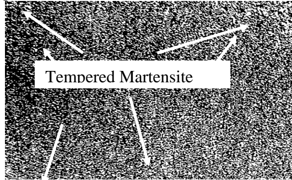
Figure 3.2. Microstructure of the Sample Subjected to DCT
