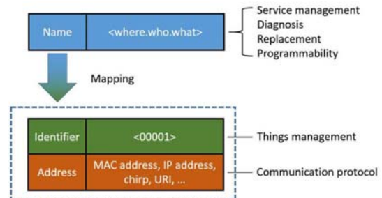
Fig. 3. Naming mechanism in edgeOS.
