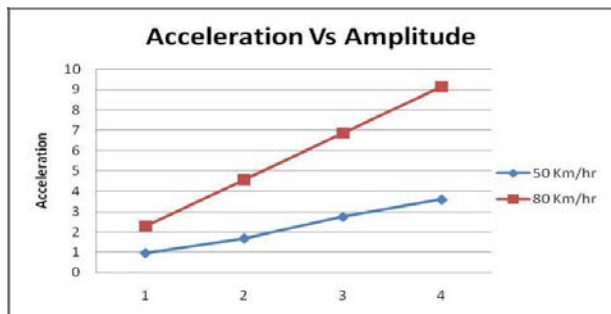
Chart -2: Amplitude Vs Acceleration
