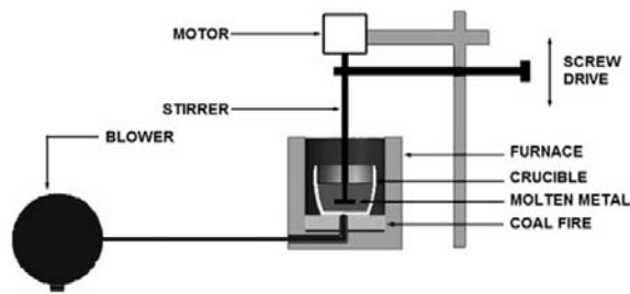
Fig.1: Basic stir casting process [8]
