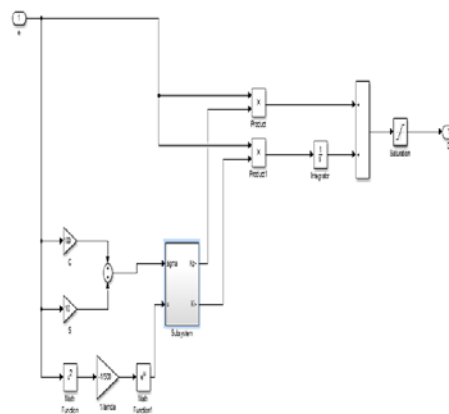
Fig.6.7: MATLAB Simulink model for DSM-PI controller
