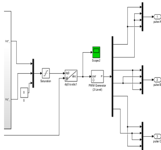
Fig. 6.5: Pulse generation for HSAPF IGBTs
