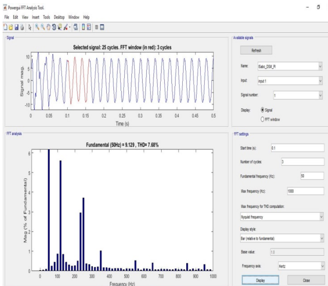
Fig 6.14 FFT analysis of DSM-PI controller at 0.1 sec
