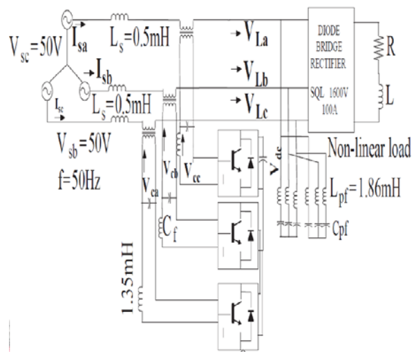
Fig.3.1: Proposed topology
