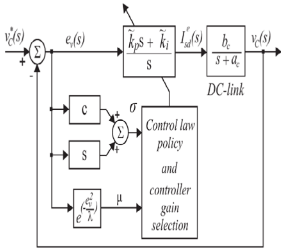
Fig.5.1: Block diagram of the DSM – PI control scheme.
