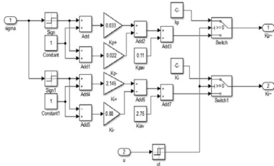
Fig.6.8: MATLAB Simulink model for DSM-PI controller developed equation
