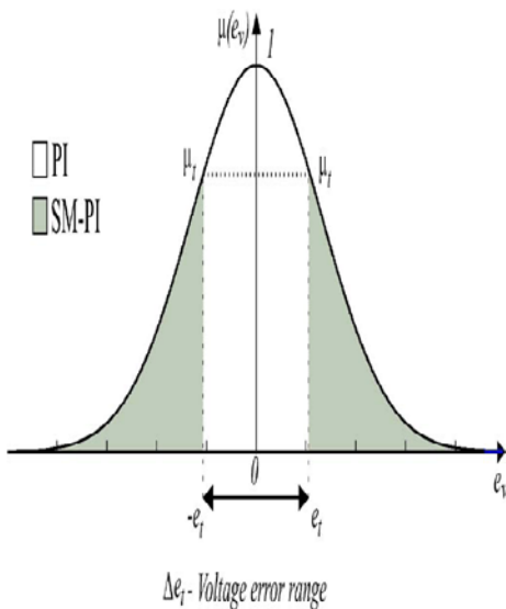
Fig 5.3 Graph of the transition criterion \mu .
