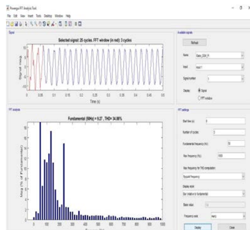
Fig 6.12 FTT analysis of DSM-PI controller at 0 sec
