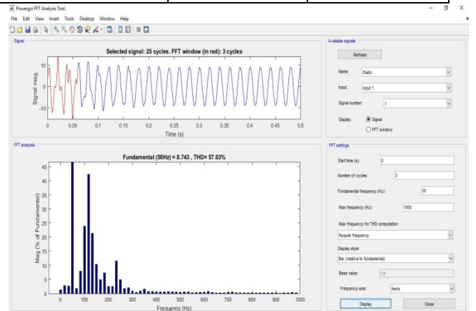
Fig 6.11 FFT analysis of SM-PI controller at 0 sec
