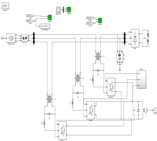
Fig.6.4: Simulink model of test system with Dual sliding PI Mode HSAPF
