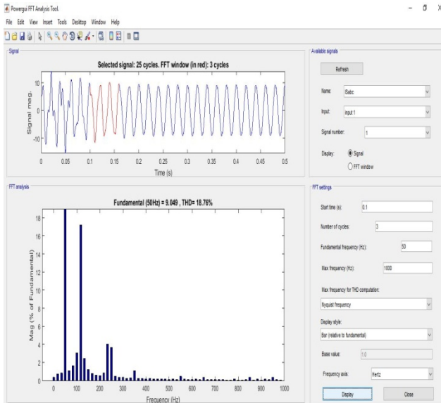
Fig 6.13 FFT analysis of SM-PI controller at 0.1 sec
