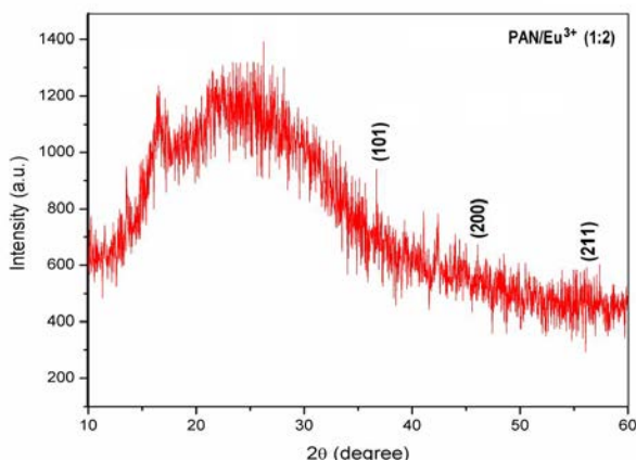
Figure 2. XRD of PAN/Eu 3+
