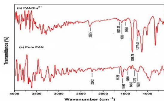
Figure 3. FTIR spectra for the PAN nanofibers and PAN/Eu 3+ (1:2) nanofibers
