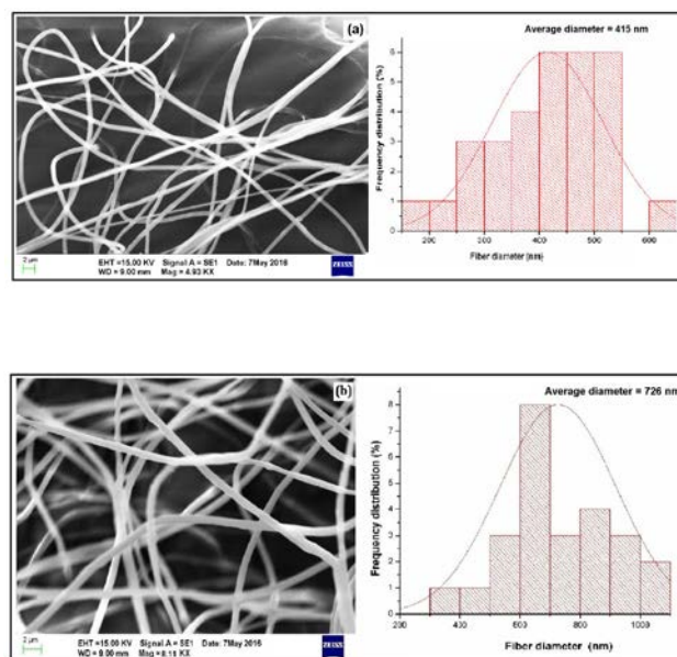
Figure 1. SEM images and histogram of electrospun nanofibers (a) \text{PAN}/\text{Eu}^{3+} (1:10) and (b) \text{PAN}/\text{Eu}^{3+} (1:2)
