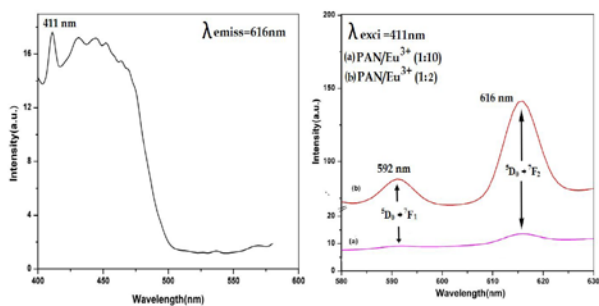
Figure 4. Excitation and emission spectra of PAN/Eu 3+ (1:10,1:2)
