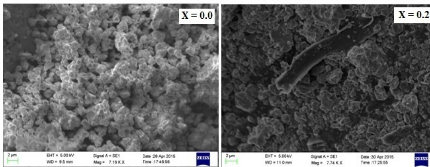
Fig. 2 SEM micrograph of \text{Ni}_{0.5-x}\text{Zn}_{0.5}\text{Cd}_x\text{Fe}_2\text{O}_4
