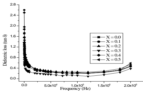
Fig. 5 Frequency dependence dielectric loss of Ni_{0.5-x}Zn_{0.5}Cd_xFe_2O_4
