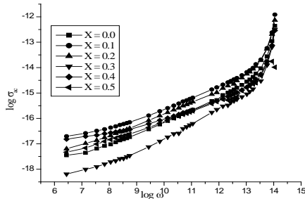
Fig. 3 Frequency dependent ac conductivity of Ni_{0.5-x}Zn_{0.5}Cd_xFe_2O_4
