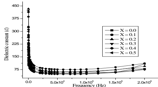
Fig. 4 Frequency dependence dielectric constant of Ni_{0.5-x}Zn_{0.5}Cd_xFe_2O_4
