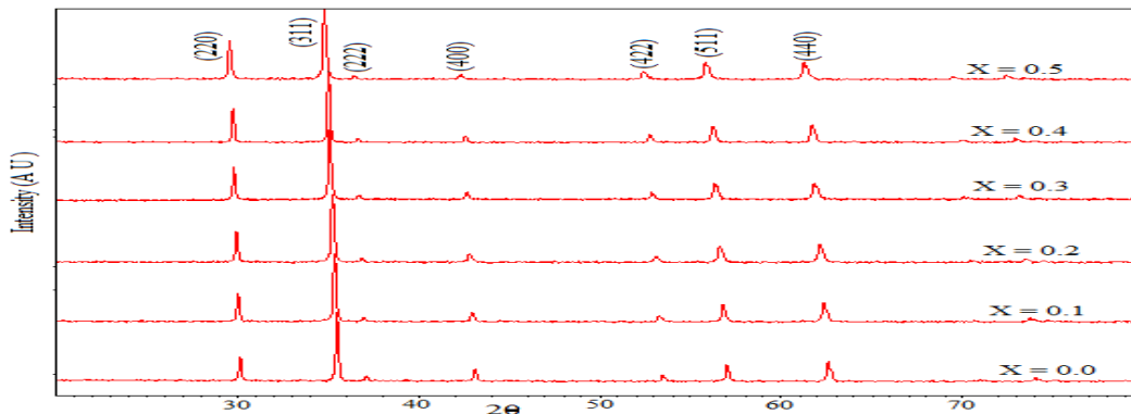
Figure 1 XRD spectra of Ni 0.5-x Cd x Zn 0.5 Fe 2 O 4
