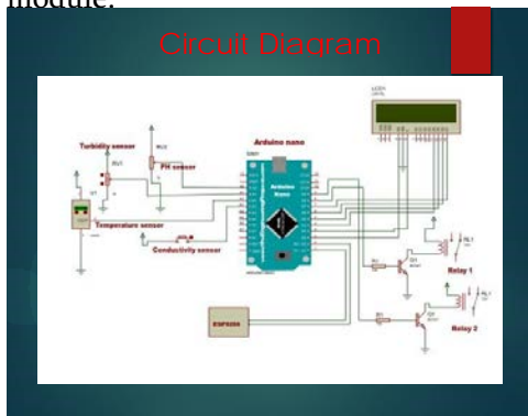
Figure1. Water Quality Implementation System
