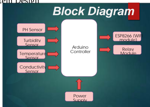
Figure 2. Water Quality Monitoring System
