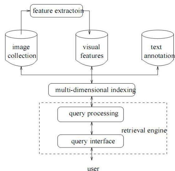
Fig: work flow diagram
