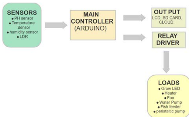
Fig.13 System architecture of smart aquaponics.
