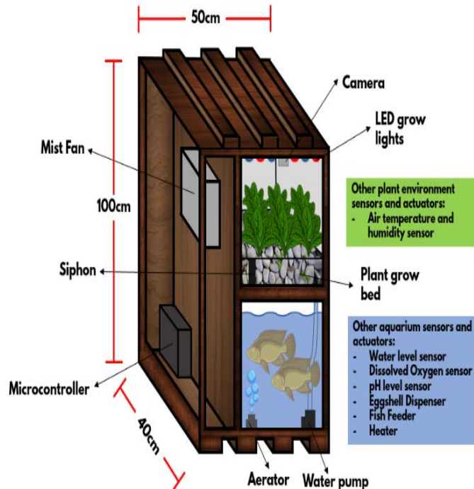
Fig. 12 conceptual picture of smart aquaponics.
